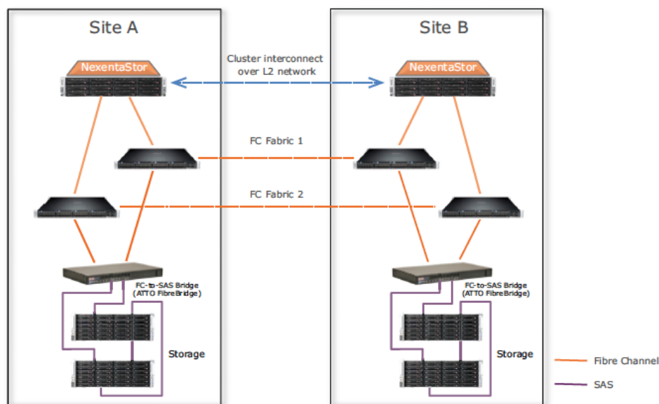
Figure 6-1 – Typical NexentaStor MetroHA Deployment with 2x ATTO FibreBridge 6500
